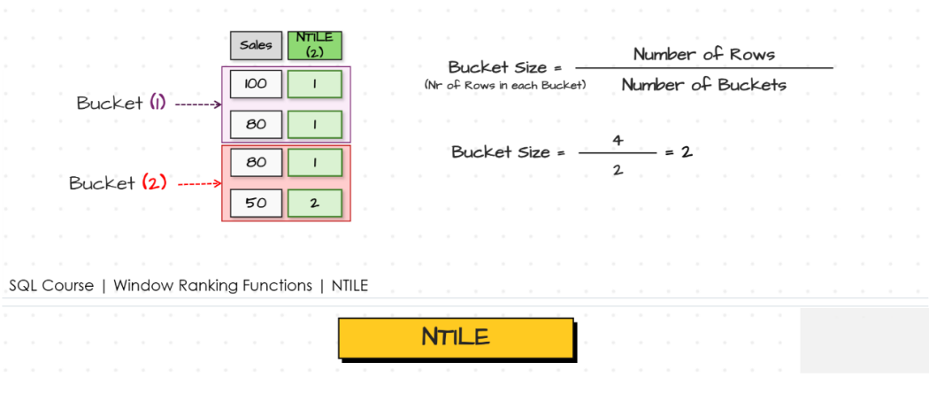
SQL Course | Window Ranking Functions | NTILE
