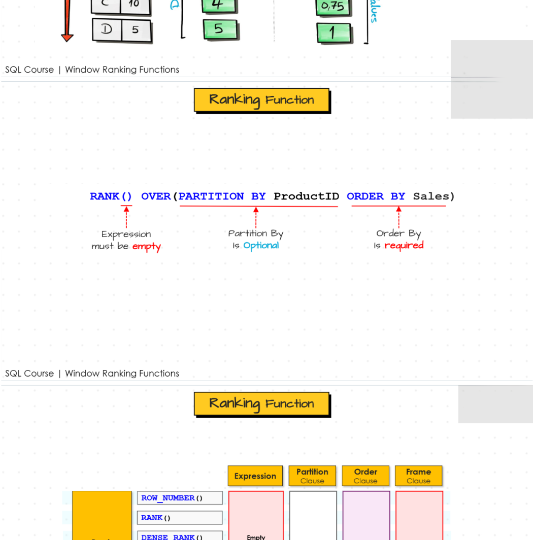
SQL Course | Window Ranking Functions
