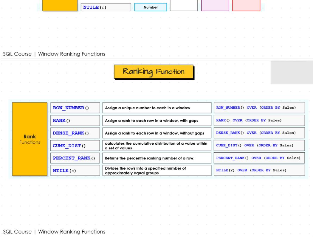
SQL Course | Window Ranking Functions
