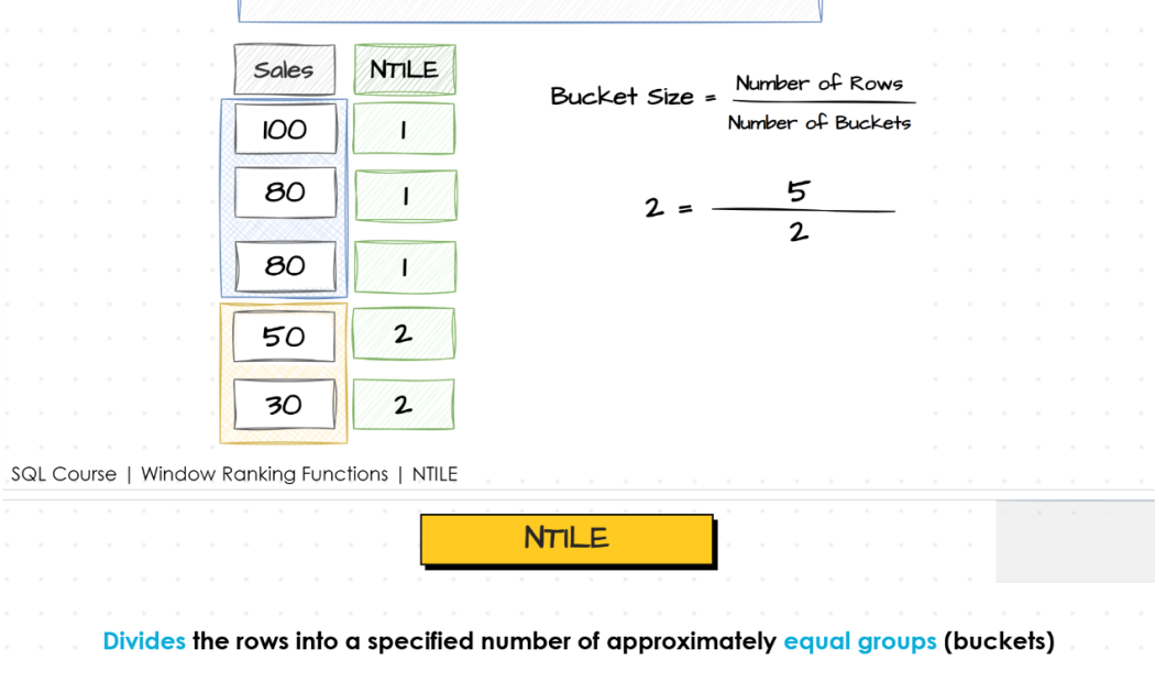
SQL Course | Window Ranking Functions | NTILE
