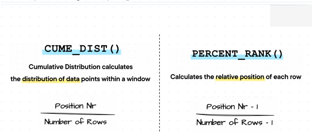
SQL Course | Window Ranking Functions | CUME_DIST & PERCENT_RANK
