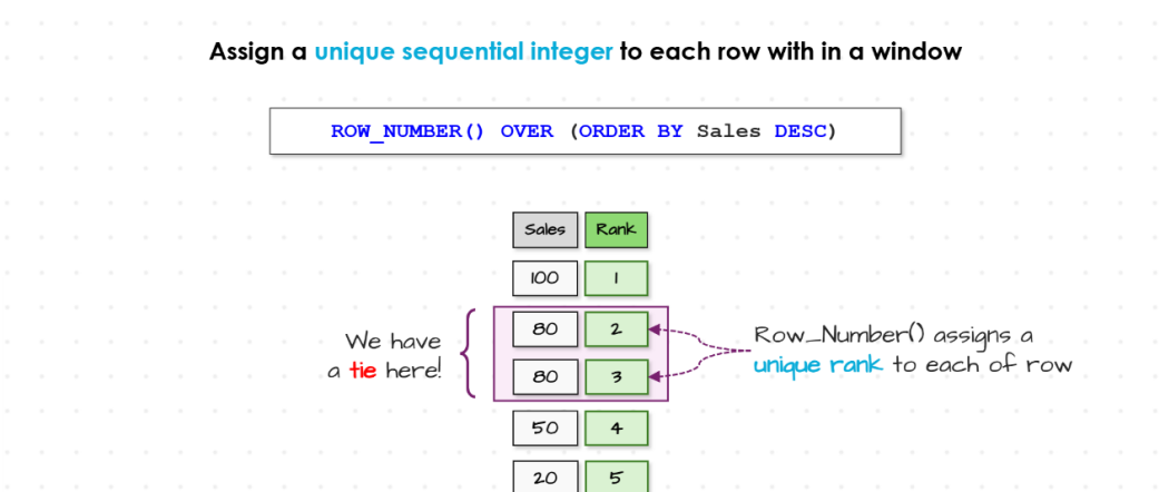
SQL Course | Window Ranking Functions
